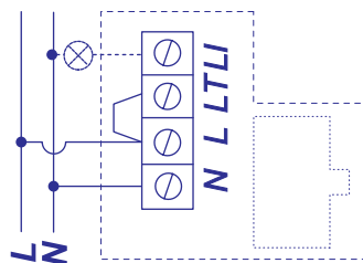
Wiring diagram 3
